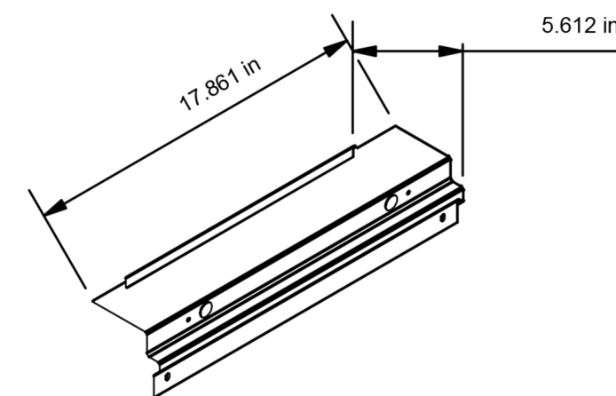
FRONT GUARD RAIL KIT
