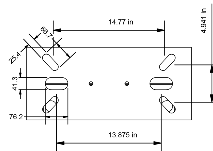
FOOT PRINT
