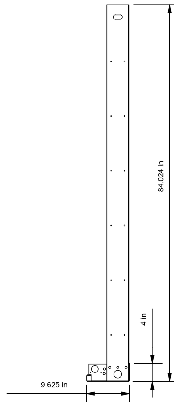
SIDE VIEW
