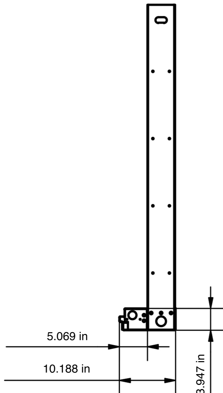
SIDE VIEW
