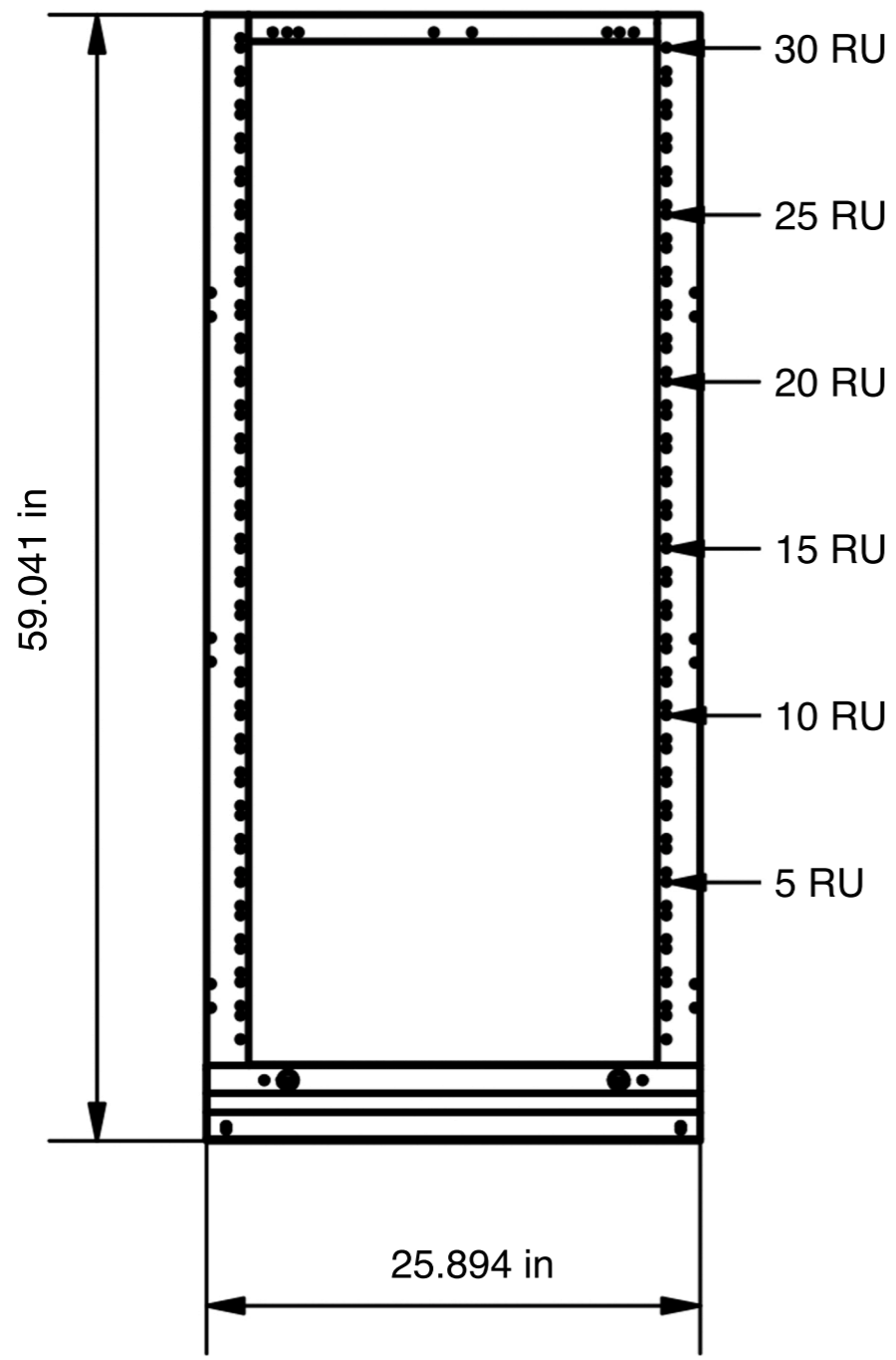
FRONT VIEW
